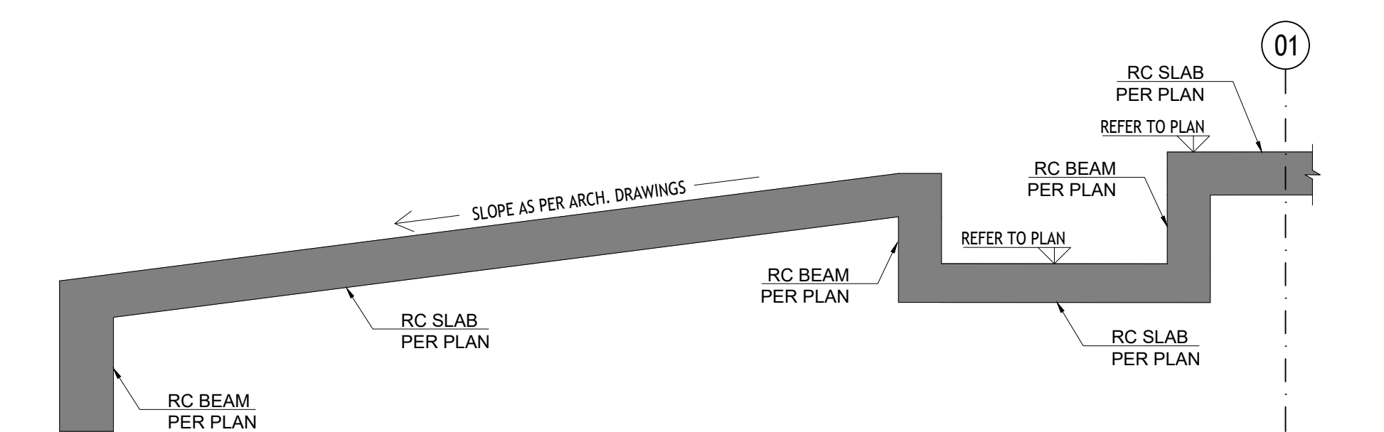
F2 TRANSFER BEAM SECTION S-102-A SCALE: 1:25
